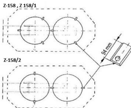
Fig. 15. Correct alternating installation of holders (knives) on working discs
