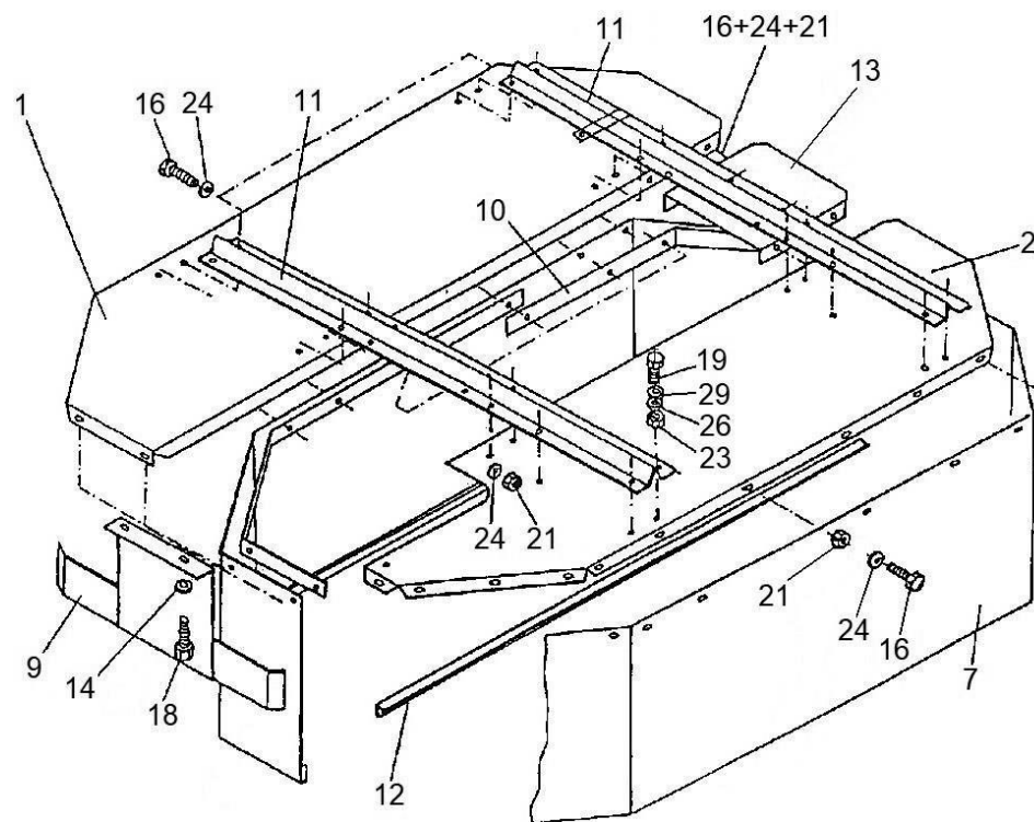
Figure K7. Metal cover set.
