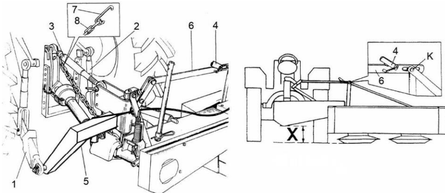
Fig. 11. Mower in correct position for operation: 1 - tractor lower link, 2 - hanger, 3 - upper connector, 4 - latch, 5 - linkage frame, 6 - tension member, 7 - chain hook, 8 - chain.
