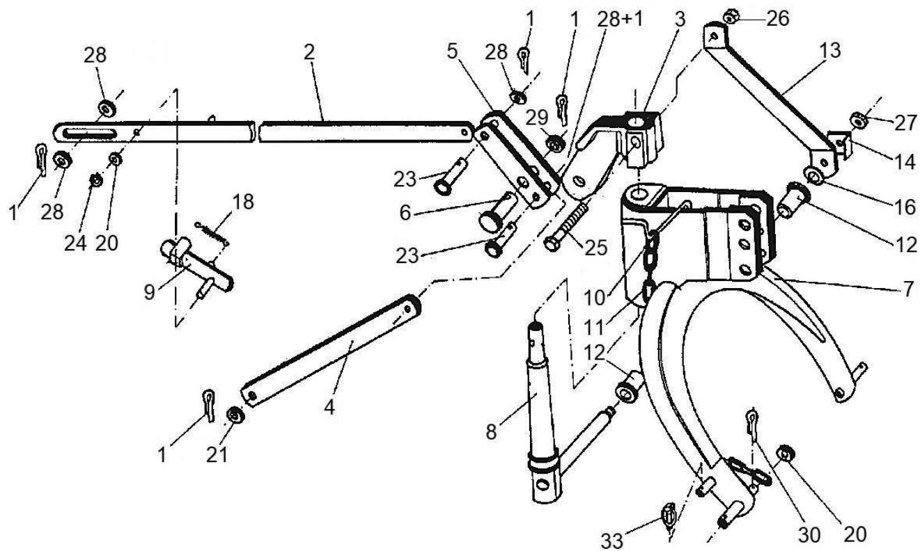
Figure K4. Linkage.
