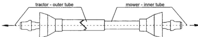
Fig. 4. U-joint shaft
