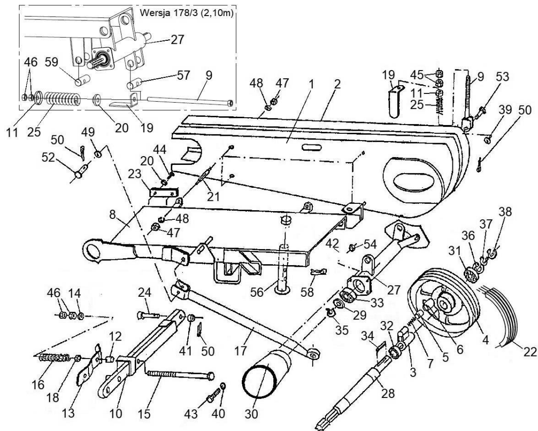
Fig. K3. Drive train and central beam
