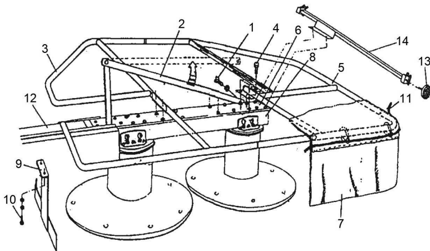
Fig. 17. Installing safety curtain: 1 - bolt M10x30, 2 - tension member, 3 - left safety curtain frame, 4 - bolt M10x25, 5 - right safety curtain frame, 6 - cover, 7 - safety curtain, 8 - main frame, 9 - side guard, 10 - bolt M8x25, 11 - cord, 12 - central beam (frame), 13 - reflector, 14 - beam with lighting holders.
