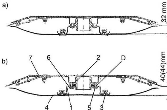
Fig. 12. Using various mowing heights: a) - low 32 mm (without spacer ring D, b) - medium 40 mm with mounted spacer ring D of 8 mm in thickness or (44 mm) with mounted spacer ring D of 12 mm in thickness; 1 - resistance disc, 2 - hub, 3 - special bolt M12 x 25, 4 - sliding disc, 5 - bolt M10 x 30, 6 - tab washer, 7 - resistance disc.
