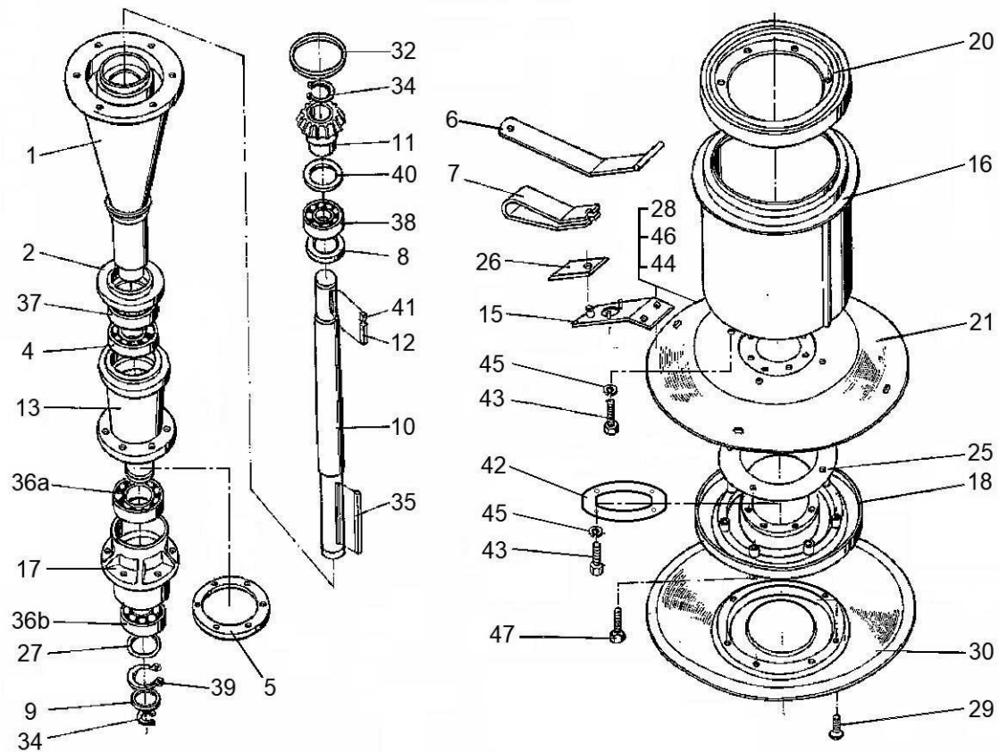
Figure K2. Cutting unit and bearings.
