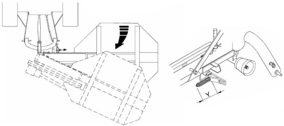
Fig. 13. Operation of safety device preventing machine damage.
