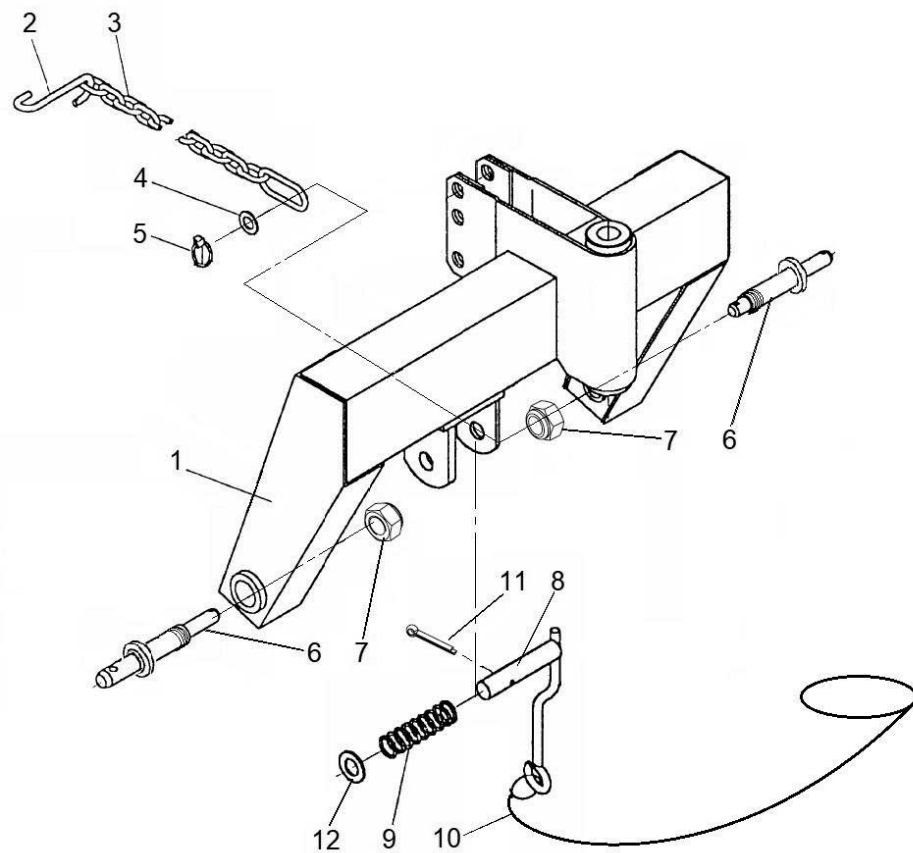
Figure K5. Linkage with replaceable pins.
