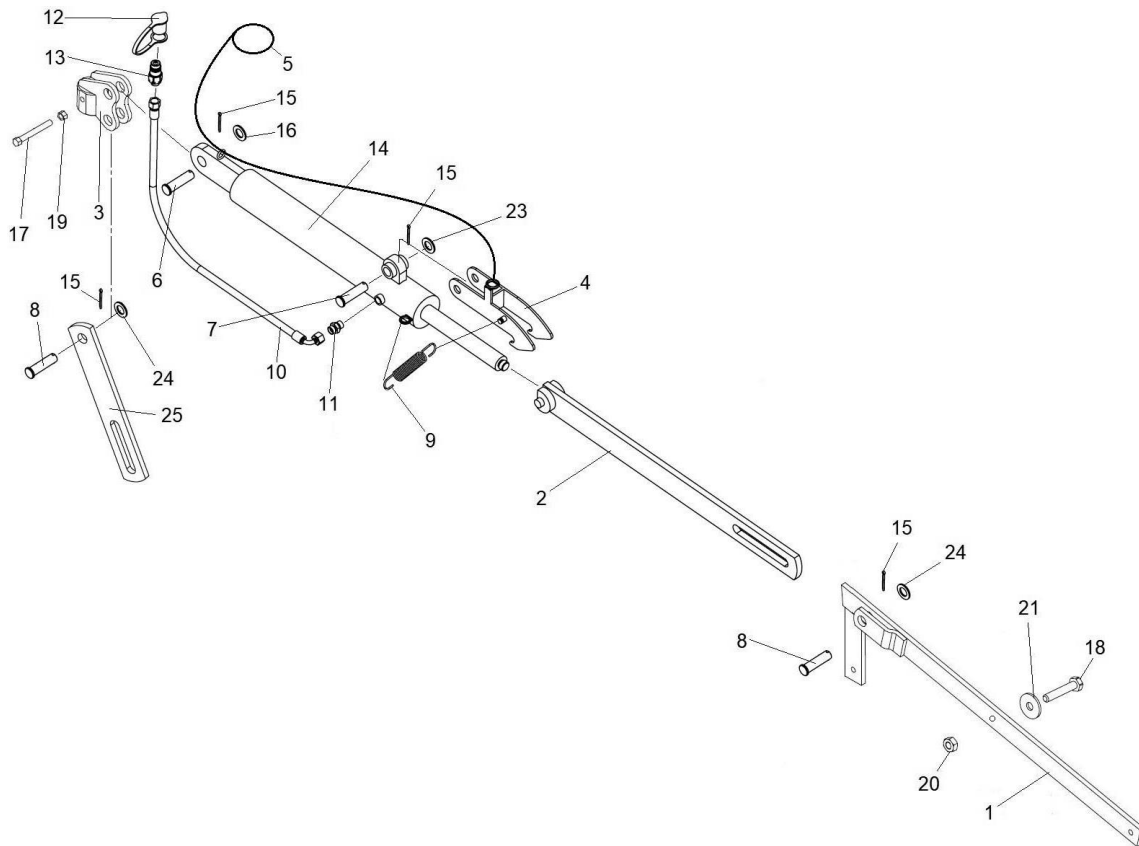
Figure K6. Hydraulic lifting system.
