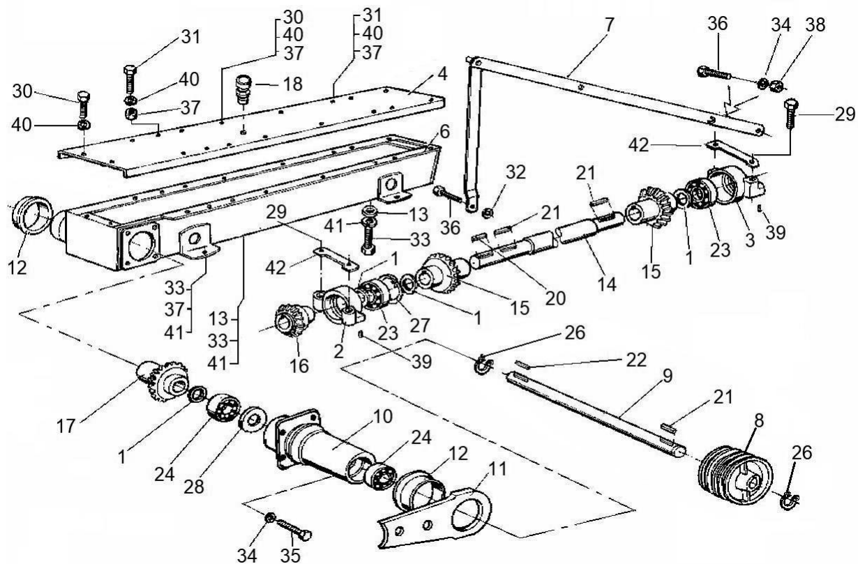
Figure K1. Main frame body and cutting unit drive.
