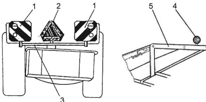
Fig. 6. Mower marking and lighting: 1 - warning light plates, 2 - warning triangle for slow-moving vehicles, 3 - special beam with holders, 4 - side reflector lights, 5 - link.
