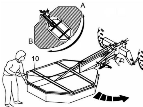
Fig. 10. Turning Z-178/3 mower: A - working position, B - transport position; 10 - latching mechanism's rope.
