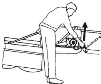
Fig. 8. Supporting mower when removing transport beam.
