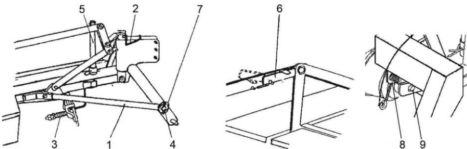
Fig. 5. Mower in transport position: 1 - transport beam, 2 - yoke hook, 3 - safety device, 4 - upper frame pin, 5 - support, 6 - latch - transport position, 7 - linchpin, 8 - latching mechanism, 9 - safety pin.
