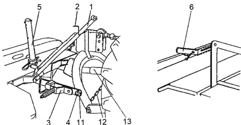
Fig. 7. Mower in working position: 1 - transport beam, 2 - yoke hook, 3 - safety device, 4 - upper pivot of linkage frame, 5 - support, 6 - latch, 7 - yoke hook, 8 - chain, 11 - linchpin, 12 - chain, 13 - U- joint shaft.
