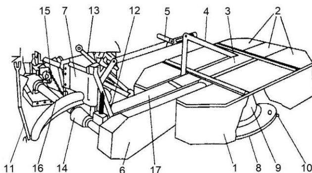
Fig. 1. Rotary mower Z-158: 1 - safety curtain, 2 - curtain frame, 3 - main frame, 4 - tension member, 5 - latch, 6 - guard, 7 - linkage frame, 8 - sliding disc, 9 - working drum, 10 - knife, 11 - tractor lower link, 12 - safety device, 13 - transport beam, 14 - roof guard, 15 - safety chain, 16 - U-joint shaft, 17 - central frame.
