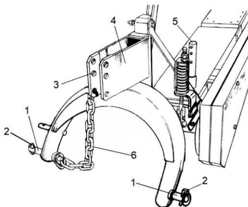
Fig. 3. Mower linkage frame: 1 - linkage frame lower pivot, 2 - linchpin, 3 - openings in linkage frame yoke, 4 - linkage frame yoke, 5 - support, 6 - chain.
